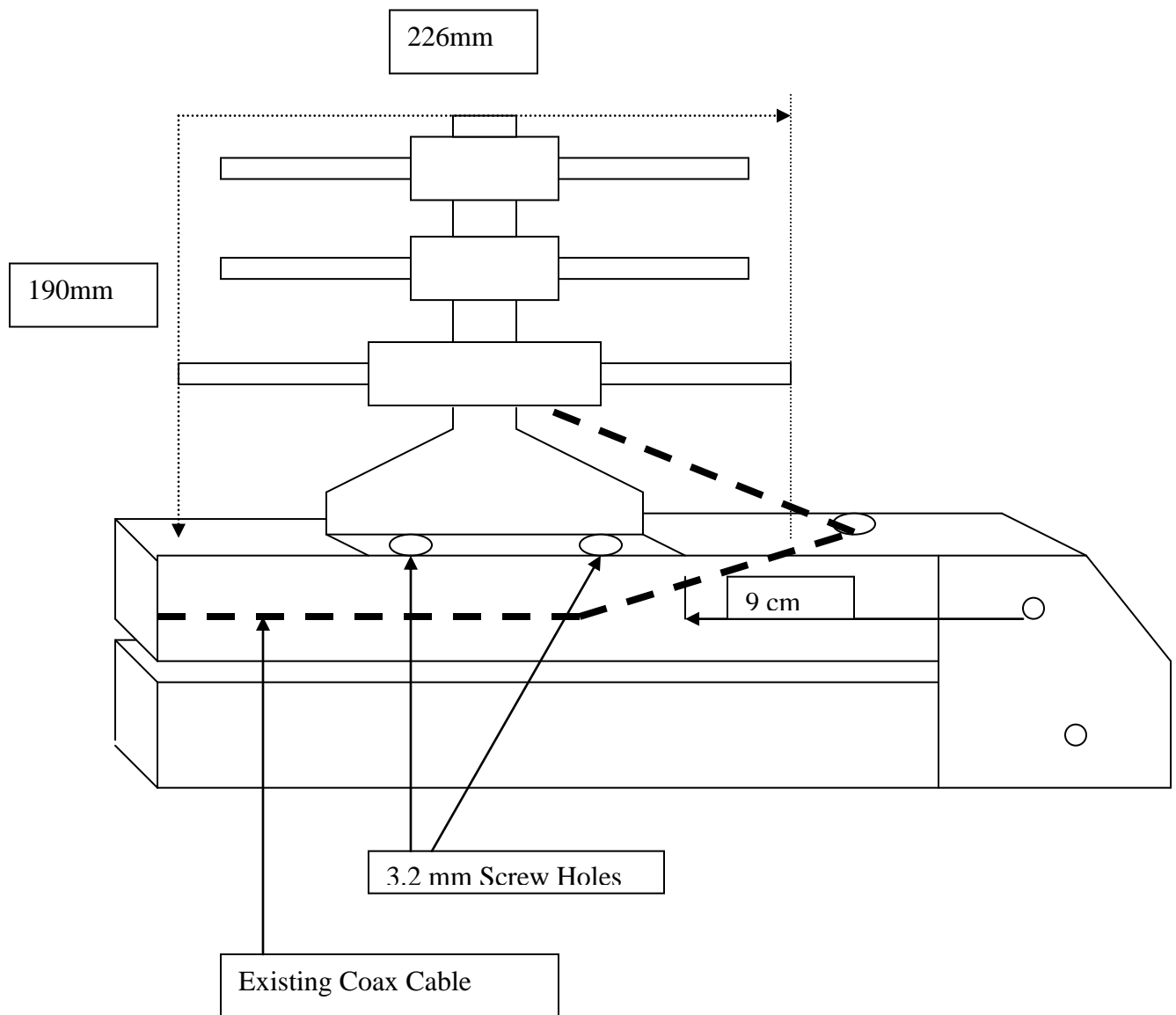
WINSIG Antenna Systems. Detail of attaching WinSig-V2.3 to Aluminium Antenna Uprights
