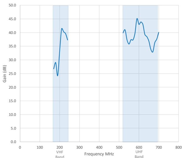
Frequency Response
